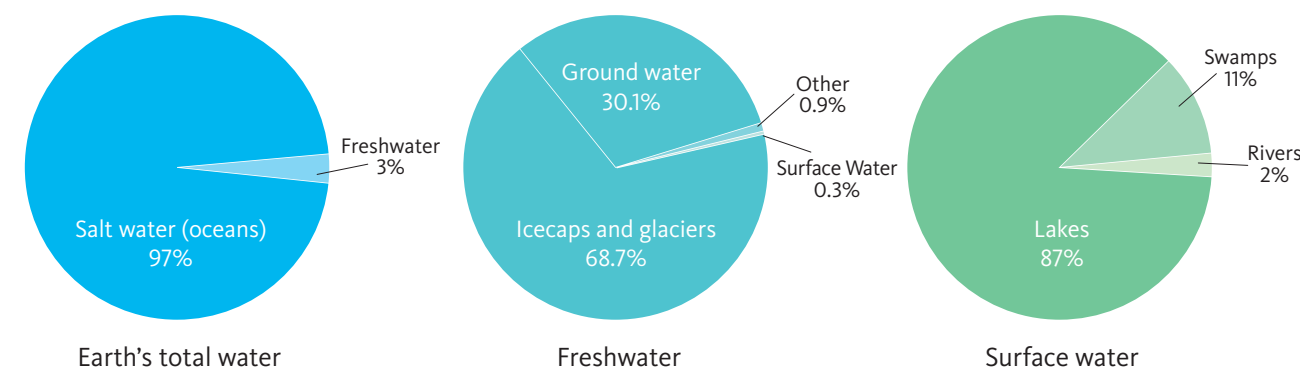
Figure 3. The distribution of water resources on Earth.
